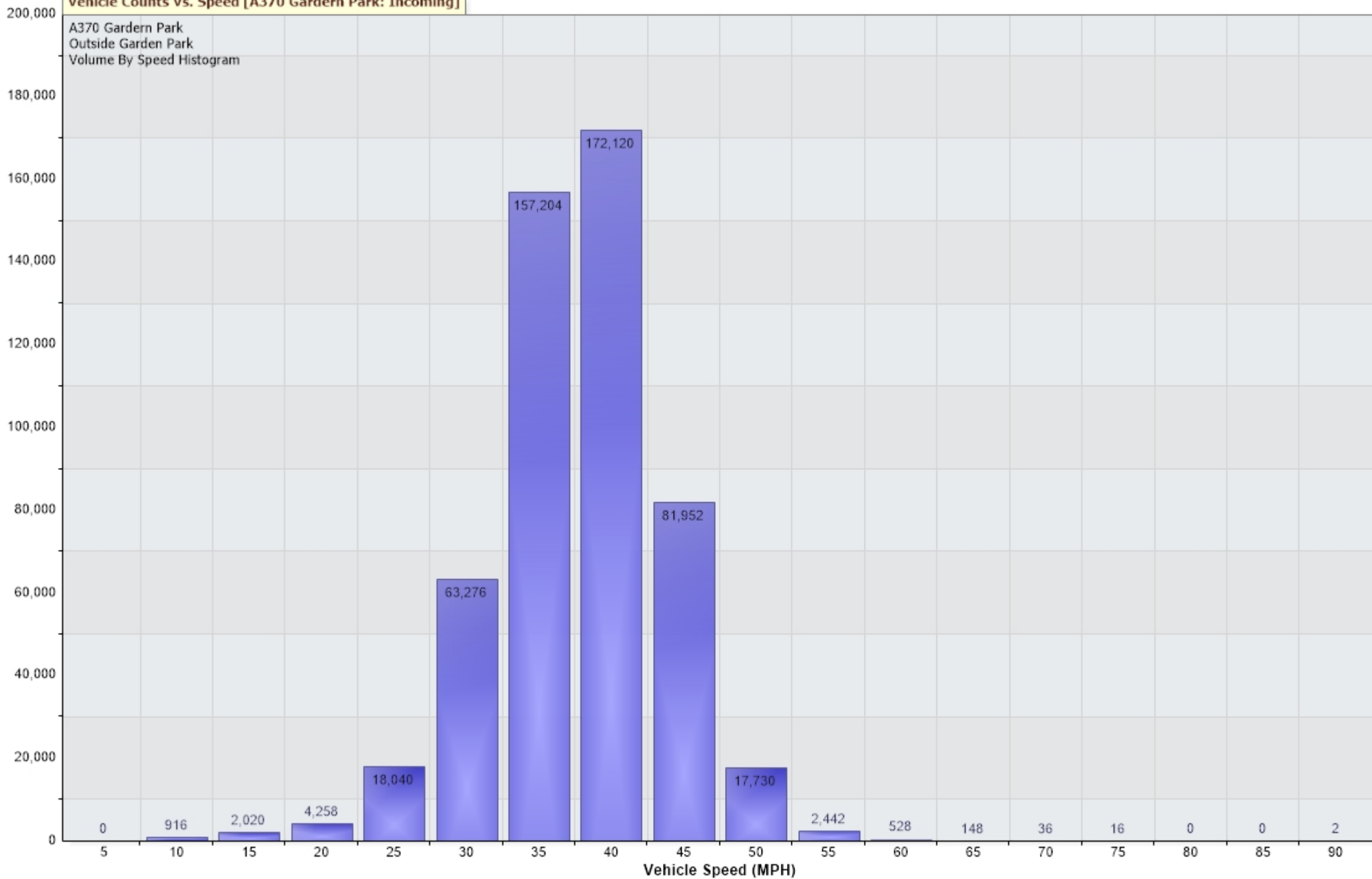
Vehicle Counts Vs. Speed [A370 Gardern Park: Incoming]
